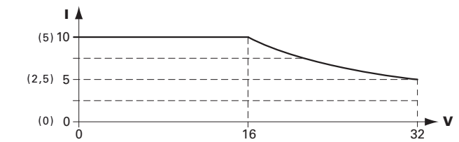
(HM2030) HM2020 power hyperbola
